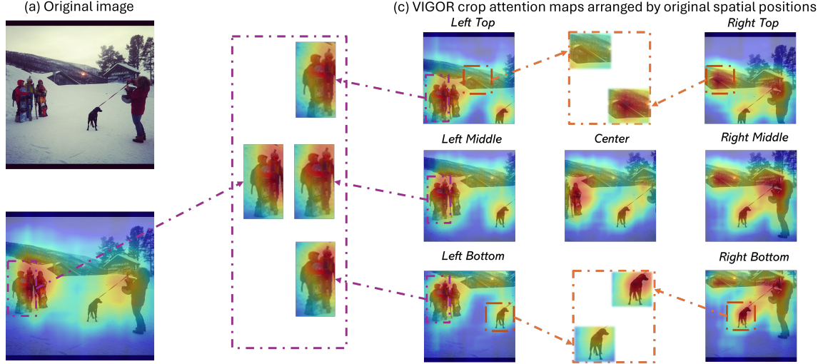
Figure 3: Case study: attention visualization on a hard instance. Base Model: LLaVA-1.5-13B; Question: Is there a backpack in the image; Ground truth: Yes; Response w/o VIGOR: No; Response w/ VIGOR: Yes. The purple dashed box highlights the comparison between the original global attention and VIGOR’s crop-based attention over the backpack region. The orange dashed boxes show attention differences across crops.
