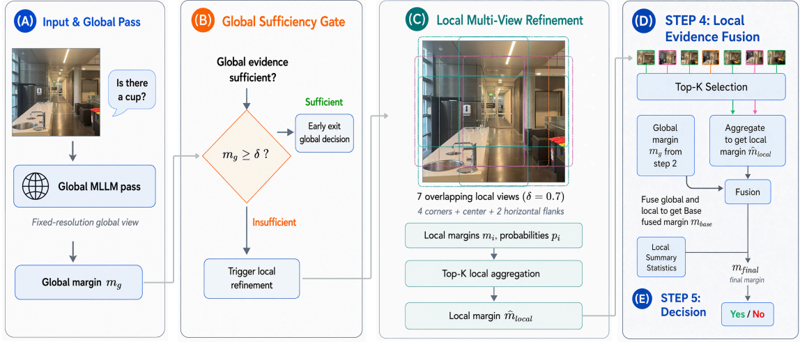
Figure 2: Overview of VIGOR. VIGOR first uses the global yes-no margin to decide whether the full-image evidence is sufficient. Routed cases are refined through seven overlapping local views, followed by top- K local aggregation, global-local evidence fusion, and asymmetric decision stabilization.
