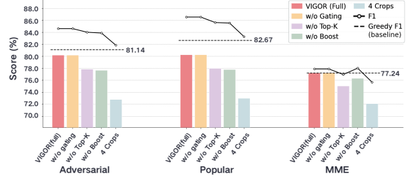
Figure 7: Ablation results of VIGOR on LLaVA-1.5-7B across POPE-Adversarial, POPE-Popular, and MME. Bars denote recall, the solid line denotes F1-score, and the dashed line indicates the Greedy baseline F1.
