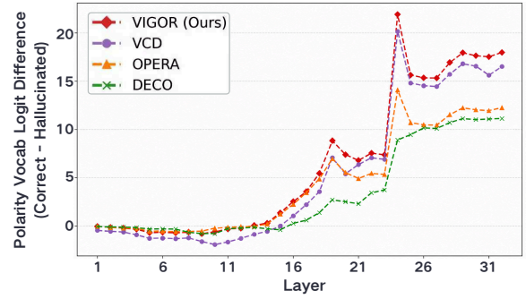
Figure 5: Layer-wise mechanistic localization analysis; Object: Residual stream; Base model: LLaVA-1.5-7B; Metric: Logit difference (correct-hallucinated); Dataset: POPE-COCO.
