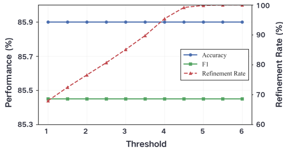
Figure 6: Effect of threshold \delta on performance and refinement rate for LLaVA-1.5-13B. Increasing \delta raises the proportion of samples sent to local refinement, while accuracy and F1 remain largely stable.
