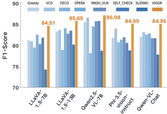
Figure 8: Performance variance analysis on POPE-COCO-Adversarial split.
