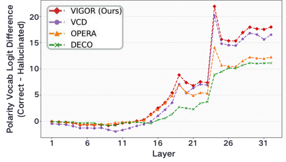
Figure 10: Layer-wise mechanistic localization analysis on POPE-COCO-Adversarial (Object: Residual stream; Base model: LLaVA-1.5-7B; Metric: Logit difference (correct - hallucinated)).
