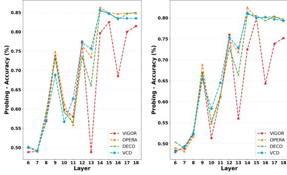
Figure 11: Layer-wise probing analysis of intermediate representations on the POPE-COCO Popular (left) and Adversarial (right) splits, using LLaVA-1.5-13B as the backbone.
