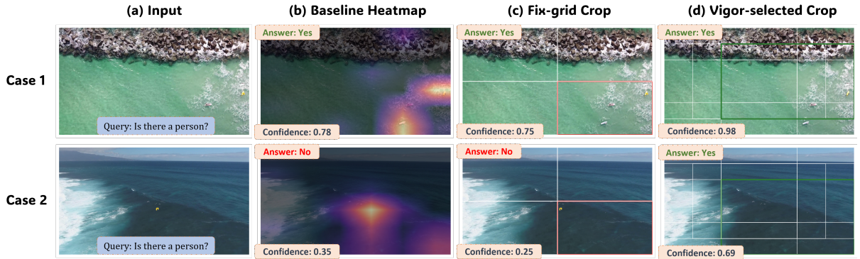
Figure 9: Qualitative comparison between the original model and VIGOR on the TinyPerson benchmark using Qwen2.5-VL-Chat. Each row shows one example. From left to right, the columns present the original image with the query, the baseline attention heatmap, the baseline grid-based crop layout, and the VIGOR crop layout. In the top example, VIGOR better preserves the tiny target within the selected local region and increases the model confidence. In the bottom example, the baseline model fails to detect the person, whereas VIGOR provides a more suitable local view and corrects the false negative prediction.
