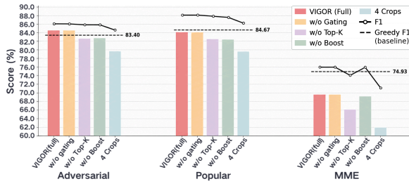
Figure 4: Ablation results on the Adversarial and Popular splits of POPE-COCO, and on MME, using LLaVA-1.5-13B as backbone model. Bars show recall, black line shows F1-score, and dashed line indicates Greedy F1 baseline.
